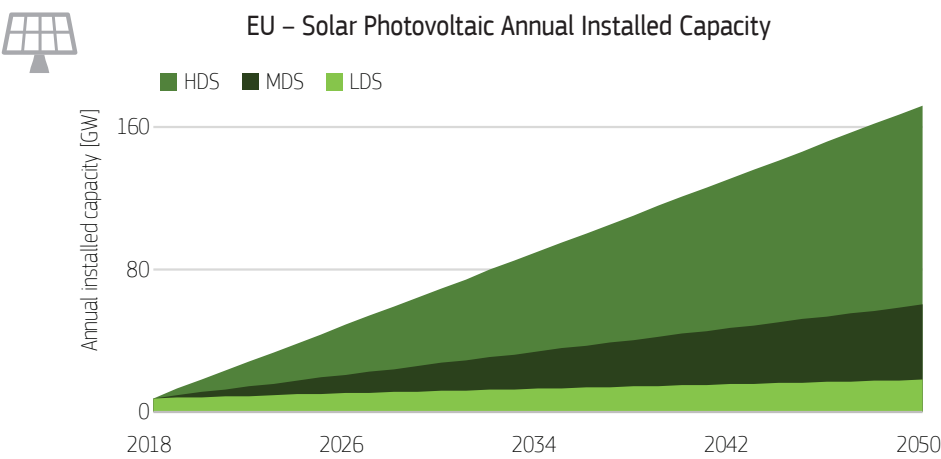
Figure 30. PV annually installed capacity in the three explored scenarios.
