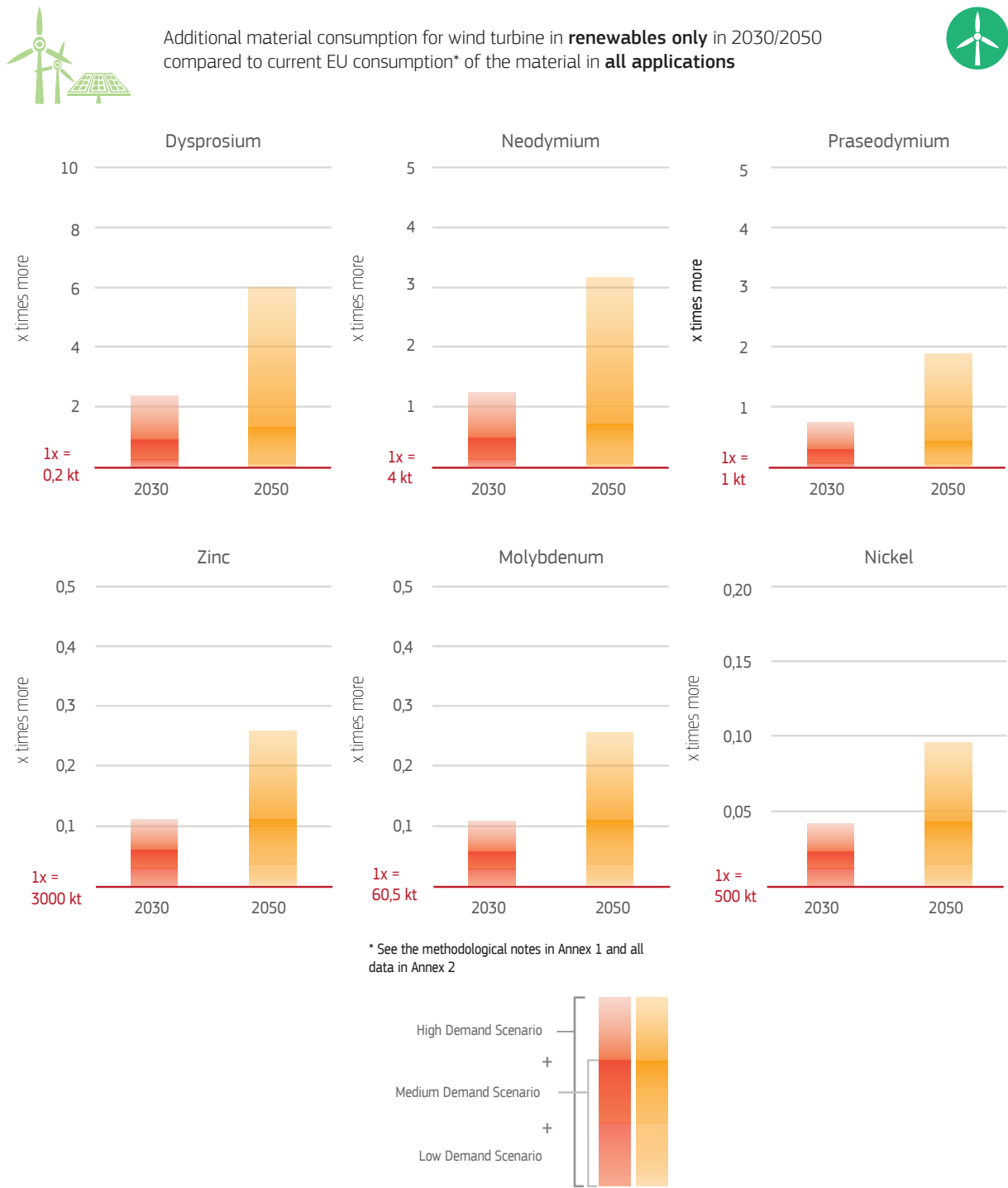
Figure 22. EU annual material demand for wind power in 2030 and 2050.
