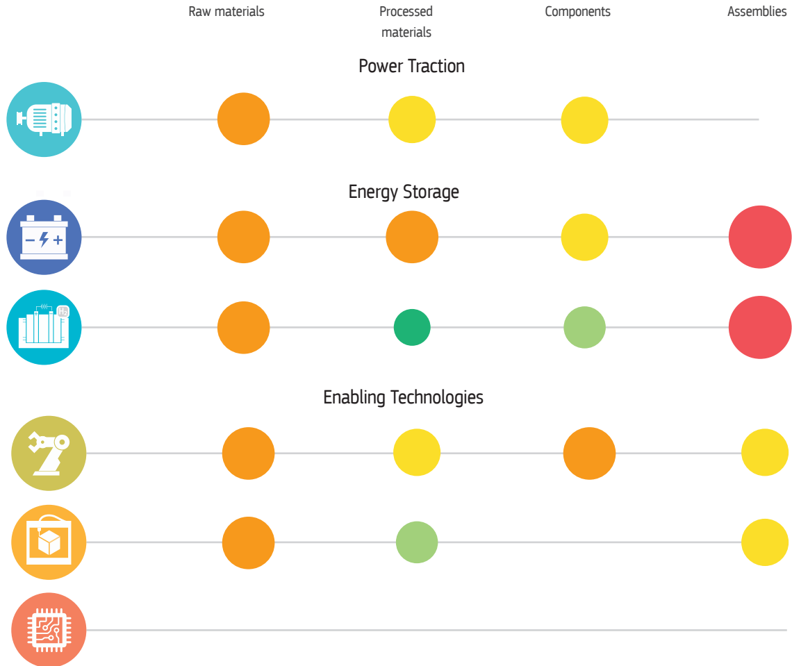
Figure 54. Potential supply risks in the value chains of emerging technologies relevant to the EU e-mobility sector: Li-ion batteries, fuel cells and traction motors
