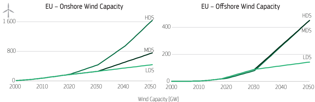
Figure 20. Onshore and offshore wind capacity in the three explored scenarios.
