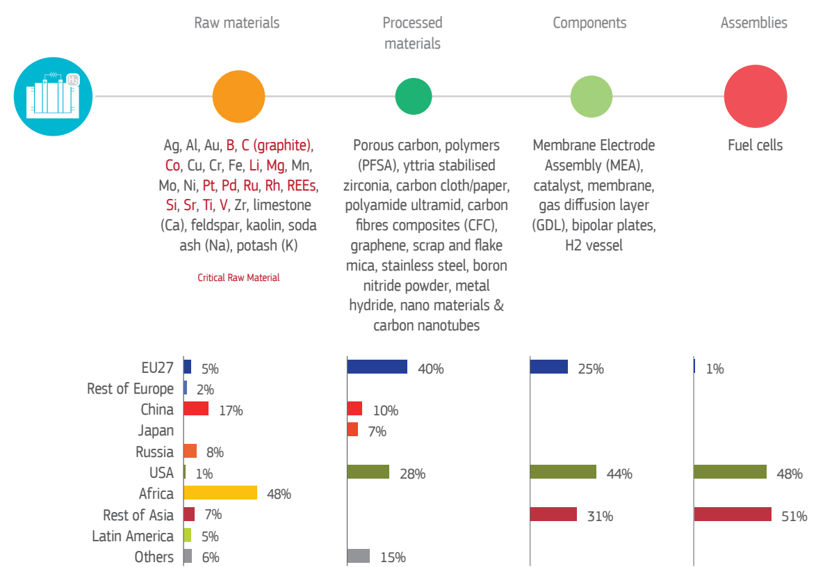
Figure 15. FCs and Hydrogen technologies: an overview of supply risks, bottlenecks and key players along the supply chain.
