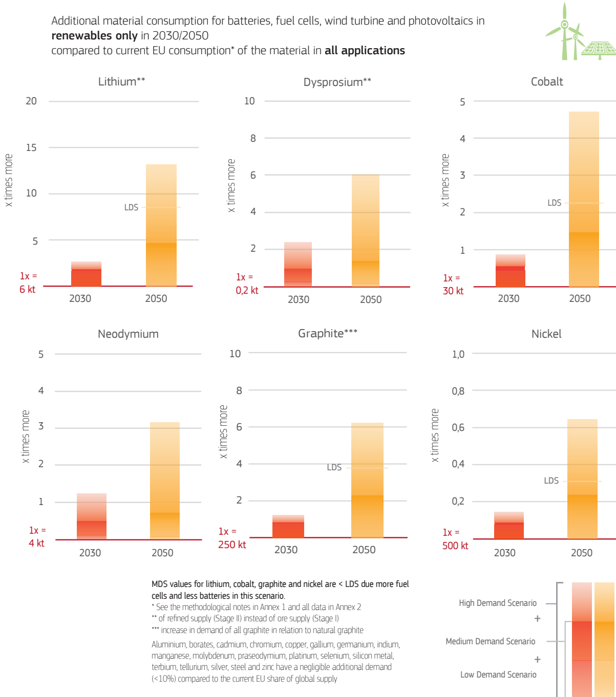
Figure 50. EU annual material demand for renewables in 2030 and 2050
